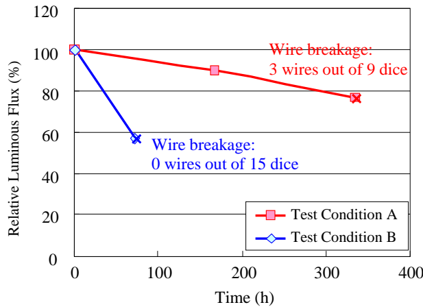
Figure 6. Reduction in Relative Luminous Flux and Occurrence of Wire Breakage in Corrosive Atmospheres
