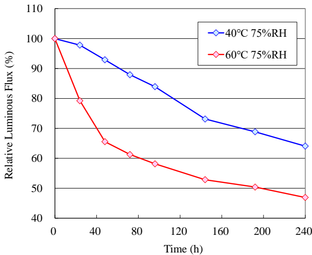
Figure 10. Lumen Maintenance for NS2W757A-V1
