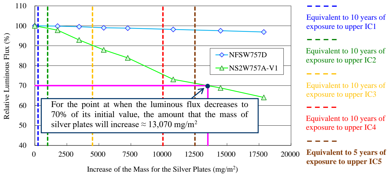
Figure 9. Estimated Lumen Maintenance Curves for NFSW757D and NS2W757A-V1
