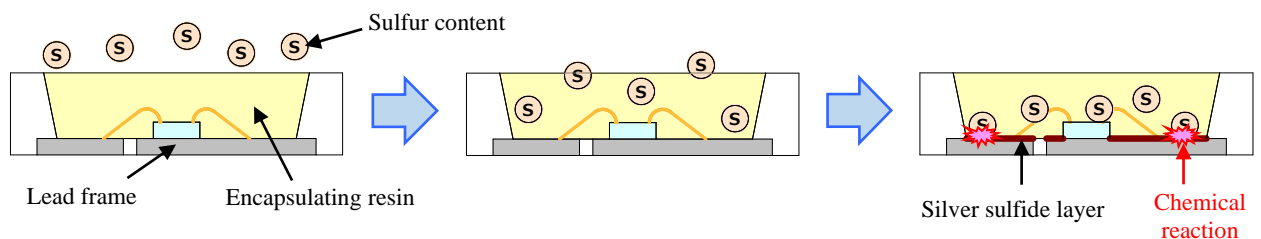
Figure 1. Schematic diagram of how sulfur causes a silver-plated lead frame to corrode (discolor)
