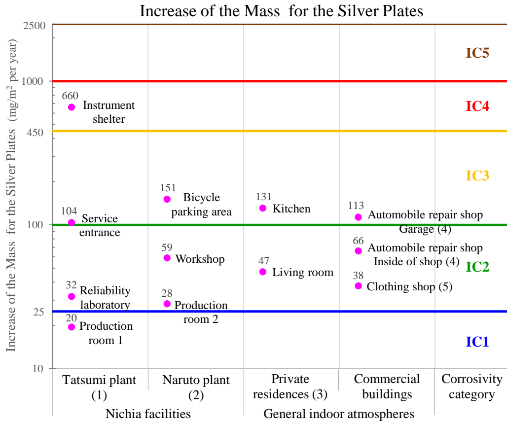
Figure 5. Field Investigation Results
