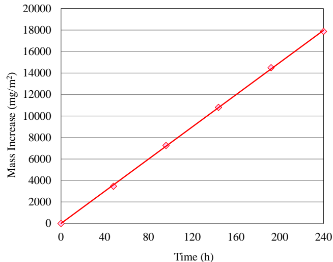
Figure 8. Increase in the Mass of the Silver Plates during the Corrosion Test
