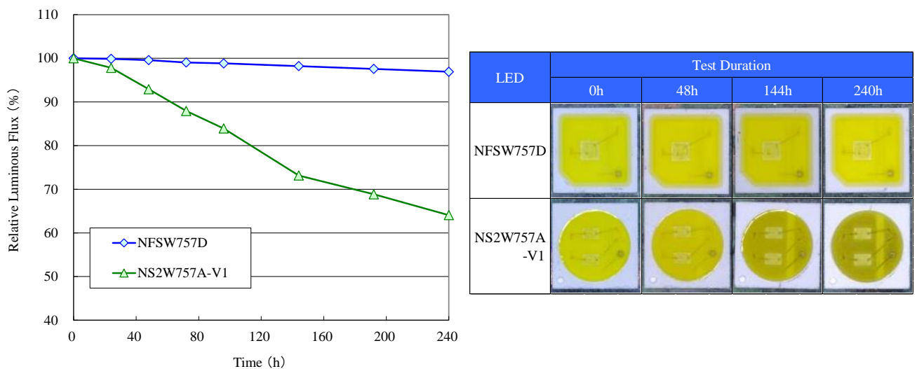
Figure 7. LED Accelerated Corrosion Test Results using the Improved Test Method
