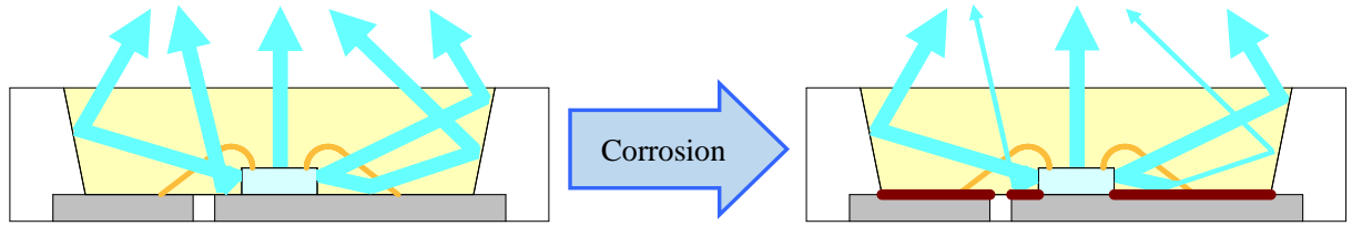
Figure 2. How the Luminous Intensity/Flux Decreases
