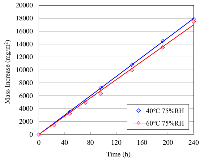
Figure 11. Increase in the Mass of the Silver Plates
